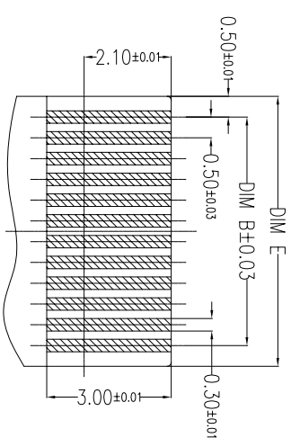
FPC LAYOUT (THICKNESS: 0.3±0.03)
